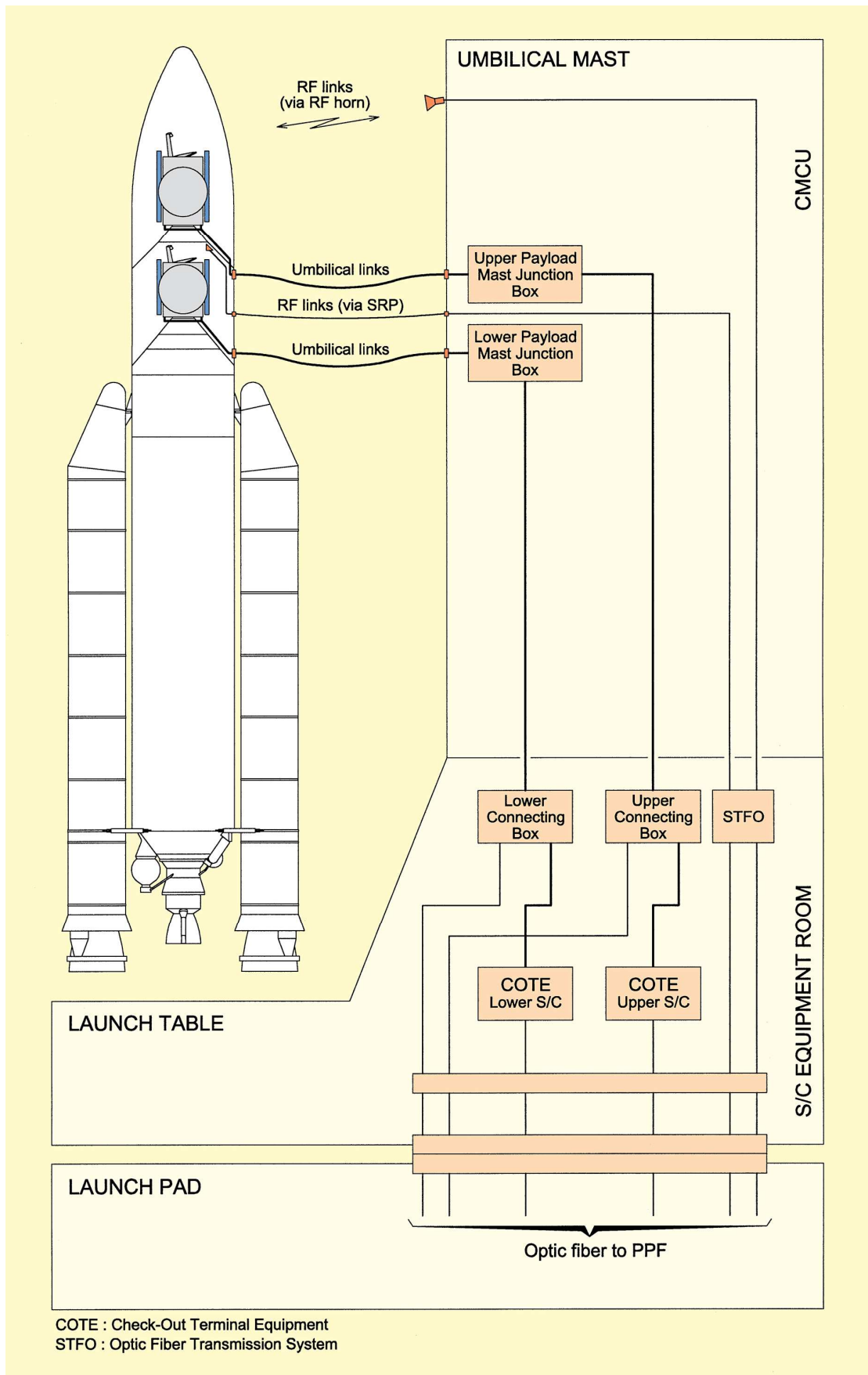
Figure 5.6.2.2.c – Principle of spacecraft / launch pad interfaces
