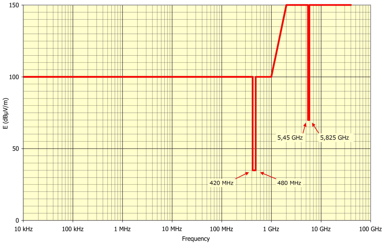
Figure 4.2.5.a – Spurious radiations acceptable to launch vehicle Narrow-band electrical field measured 1.0 m below the separation plane (free space)
